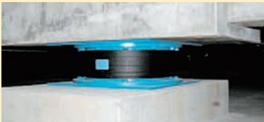
① 積層ゴム支承
